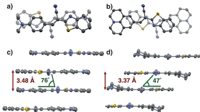
Figure 3. X-ray crystal structures of 1a and 2a drawn with thermal ellipsoids set at 50% probability and with hydrogen atoms omitted for clarity. a, b) Top view of the two nearest neighbor molecules in the crystal of 1a (a) and 2a (b). The molecules of 1a (c) and 2a (d) stack in offset columns of antiparallel dimers with displacement angles between nearest neighbors of 76° for 1a and 47° for 2a . Atom colors: C = gray; N = blue; S = yellow.
